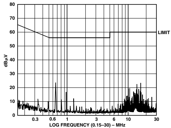
Figure 15. Conducted Emissions
